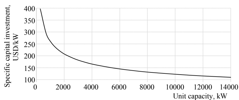
Fig. 3. Specific capital investment in AHP as a function of capacity
