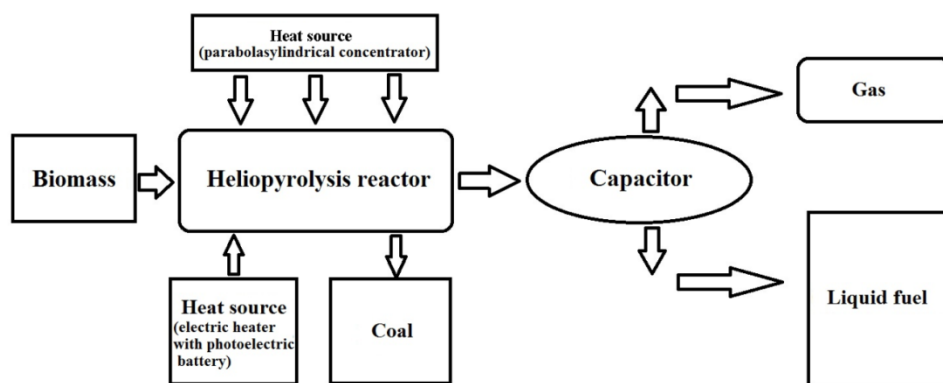
Fig. 1. Technological scheme of heliopyrolysis process
